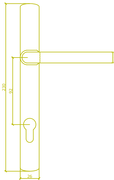
BTV (lockable balcony door without tilt)
