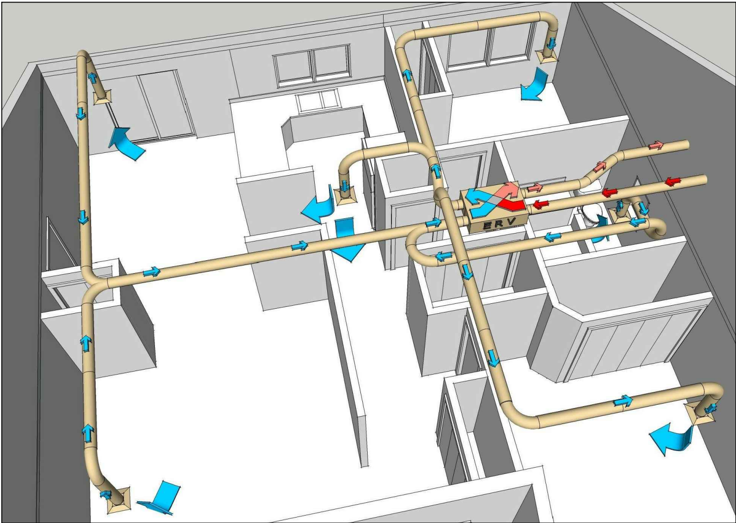
BASIC ERV SYSTEM DIAGRAM SHOWING RECOVERY OF COOLING (SUMMERTIME OPERATION)
