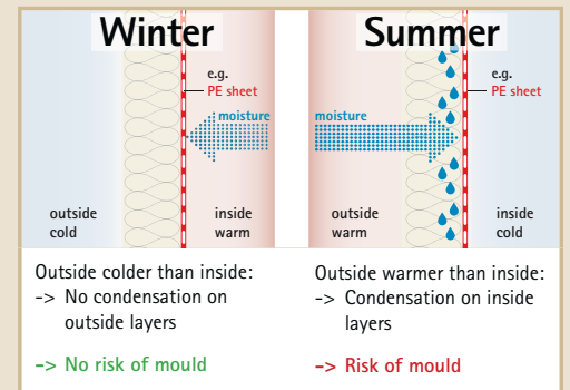
Fig. 22. The effects of a vapour retarder on the inside
