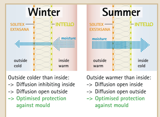
Fig. 24. The effects of intelligent moisture management
