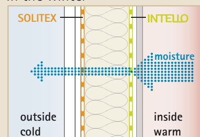
Fig. 6. Intelligent moisture management In the winter
