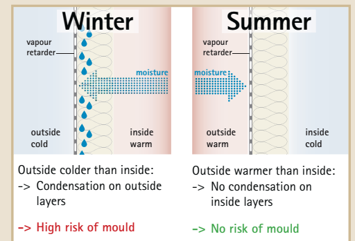
Fig. 23. The effects of a vapour retarder on the outside
