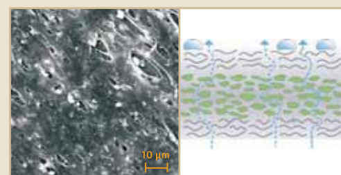
Microscopic detail of a porous membrane
