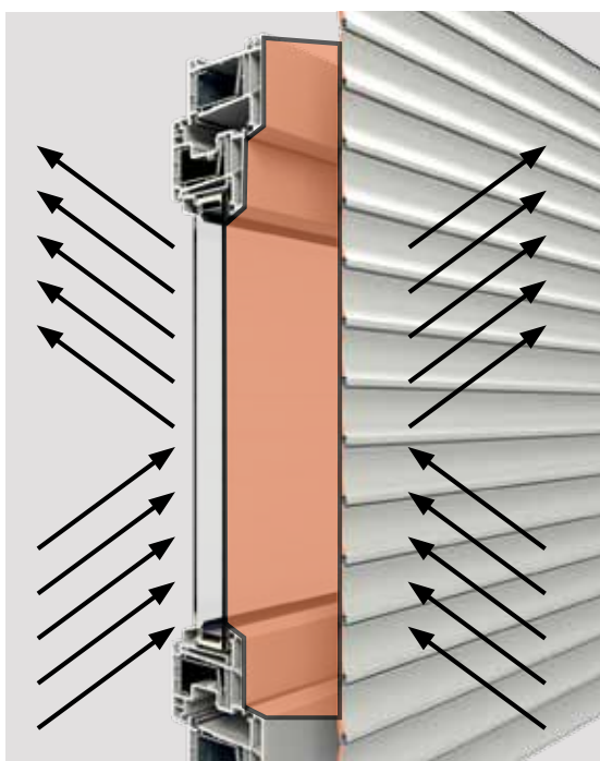
Air gap between window and roller shutter serves as insulation layer and helps to reduce heating cost.
