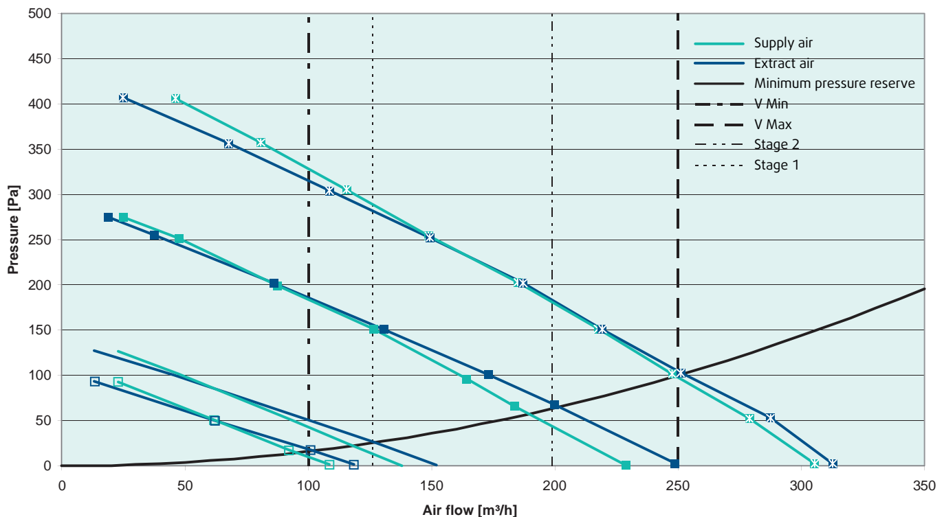
Air flow/pressure diagram
